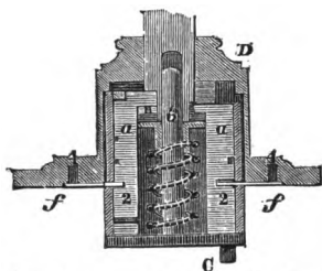
fig. 39. Section of the Bramah cylinder.
