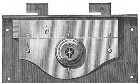
fig. 35. Exterior of a Bramah lock.
